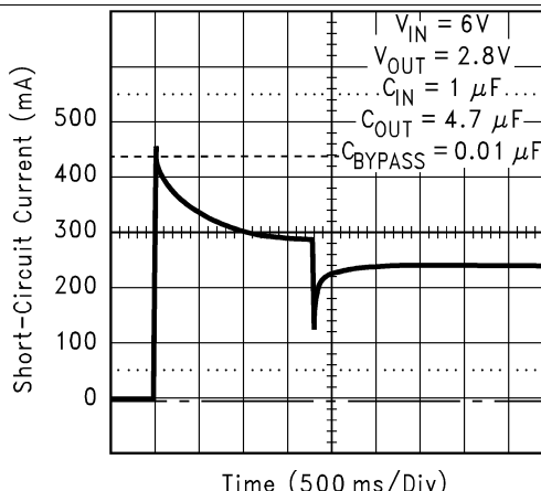
Figure 2. Short-Circuit Current
